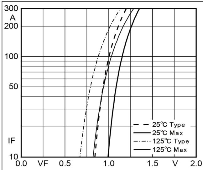
Fig5. Forward Characteristics
