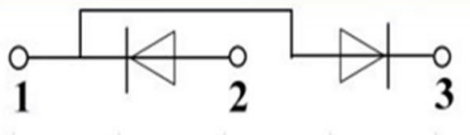
Circuit
