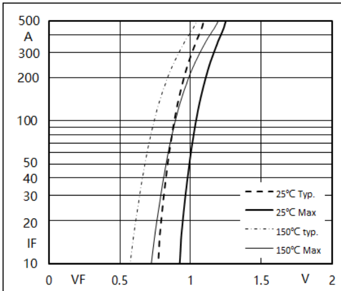
Fig5. Forward Characteristics
