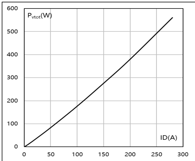
Fig1. Power dissipation
