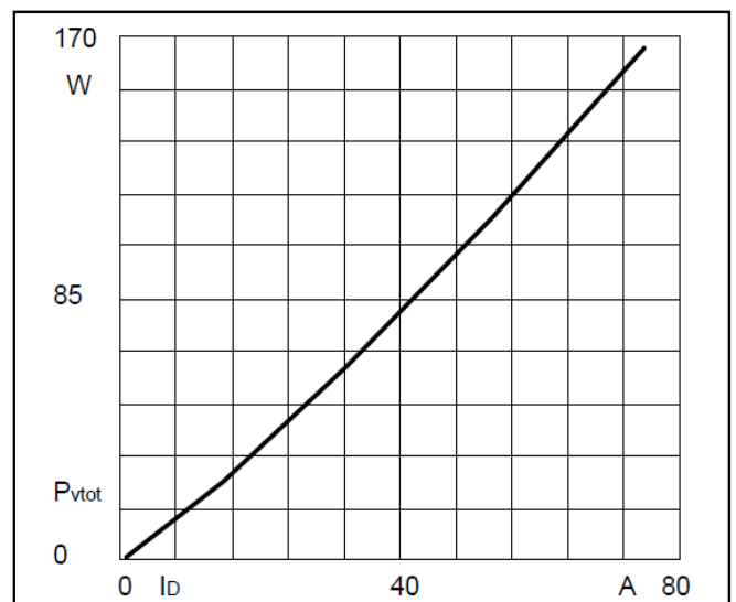
Fig2. Power dissipation
