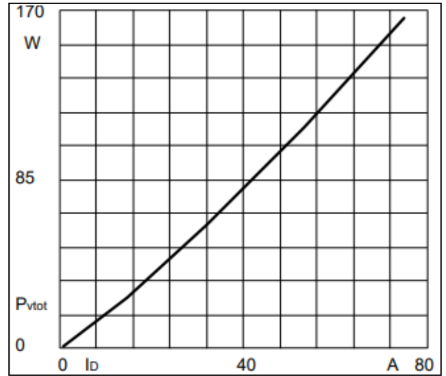
Fig2. Power dissipation
