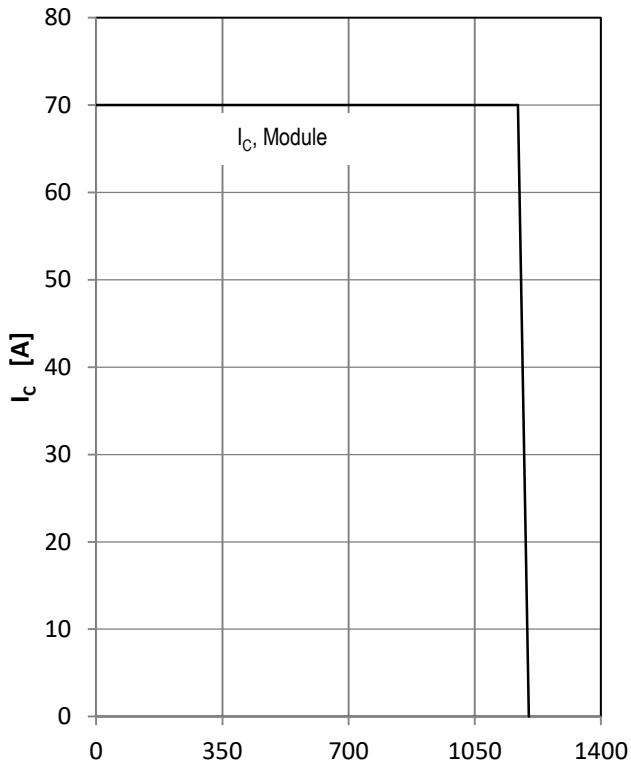
Fig5. RBSOA
