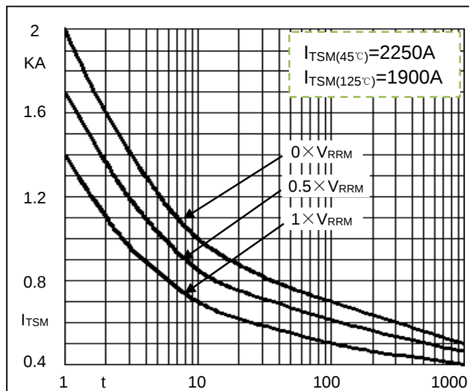
Fig5. Surge overload current vs. Cycles
