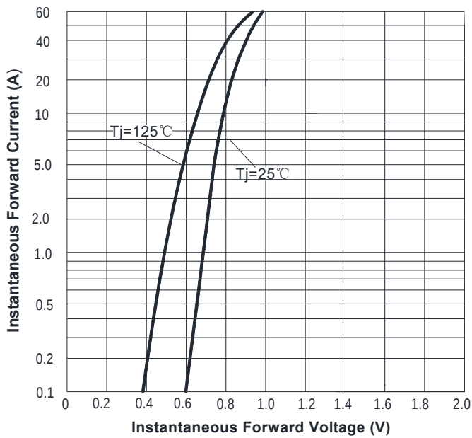
FIG3: Forward Voltage
