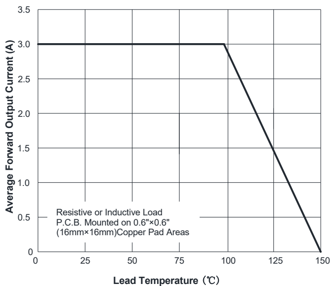
FIG.1: Io-TL Curve
