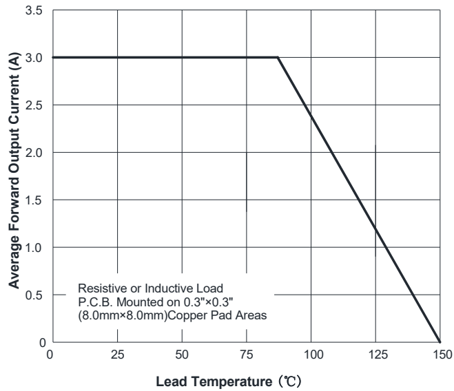
FIG.1: Io-TL Curve
