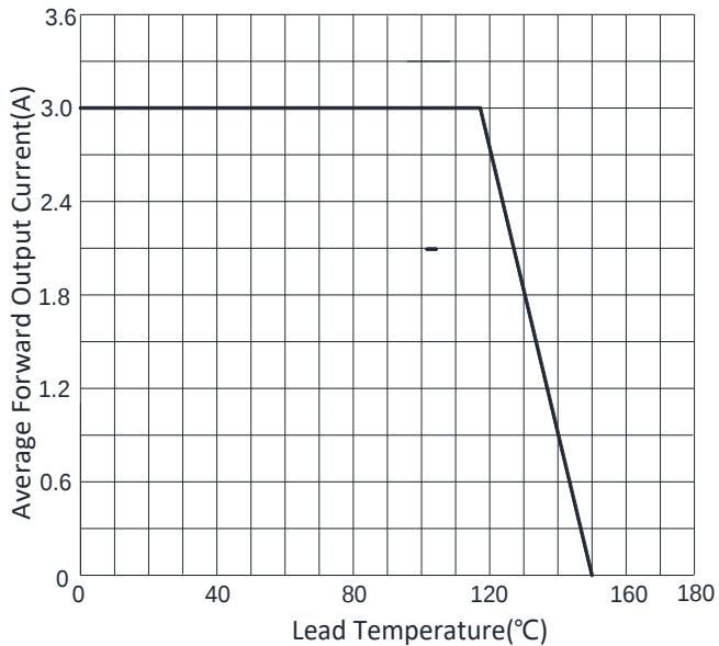
FIG1:Io-TL Curve
