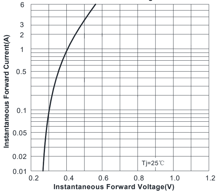
FIG3: Forward Voltage
