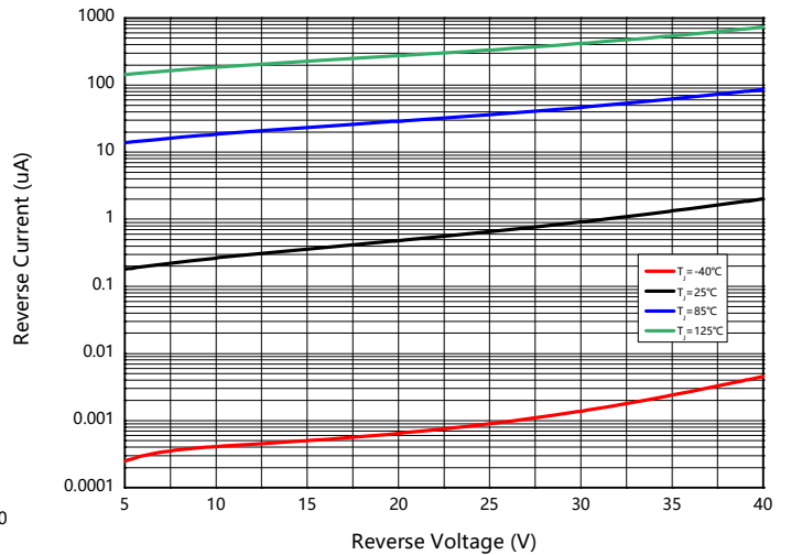
Fig.4: Reverse Characteristics
