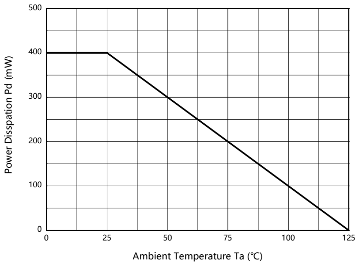
Fig.1: PD-Ta Curve
