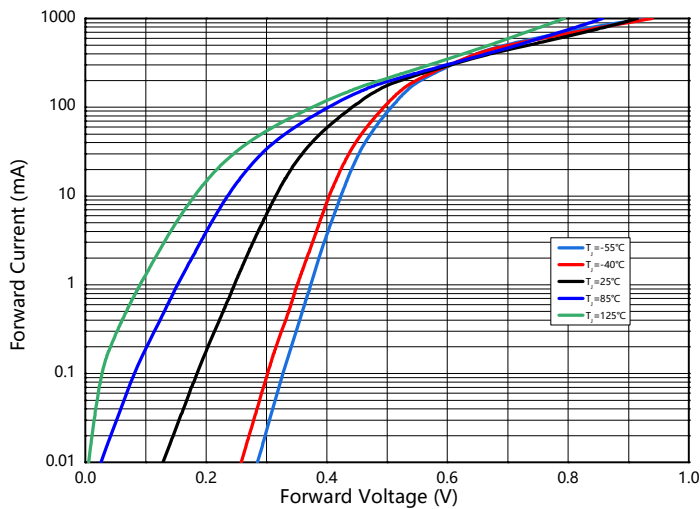
Fig.3: Forward Characteristics
