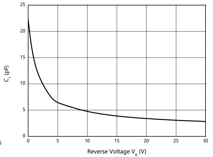
Fig.2: Capacitance Characteristics
