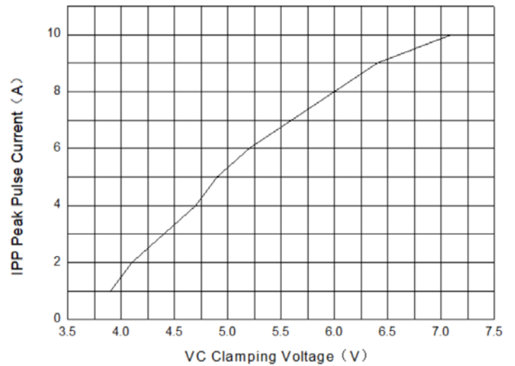
Fig2: Peak Pulse Current vs Clamping Voltage
