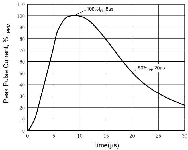
Fig.1: 8/20 \mu s Pulse Waveform
