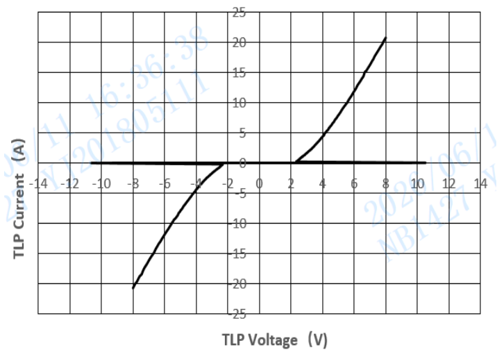
Fig 4: Transmission Line Pulsing (TLP) Plot
