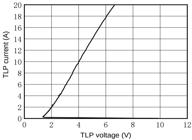
Fig. 7 TLP Measurement
