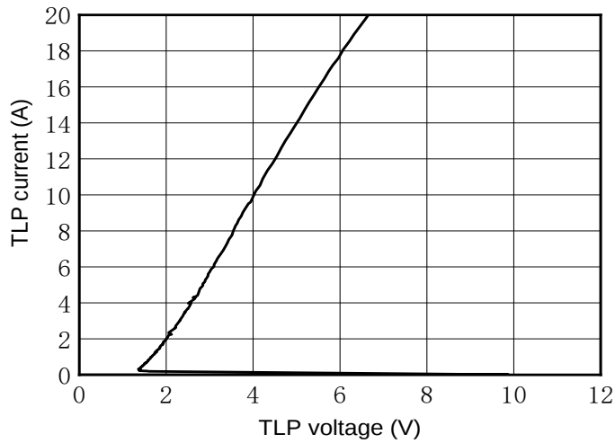
Fig.7 TLP Measurement
