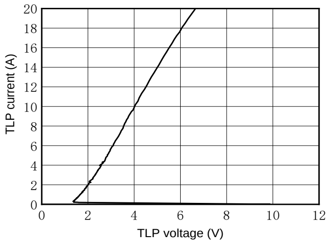
Fig.7 TLP Measurement
