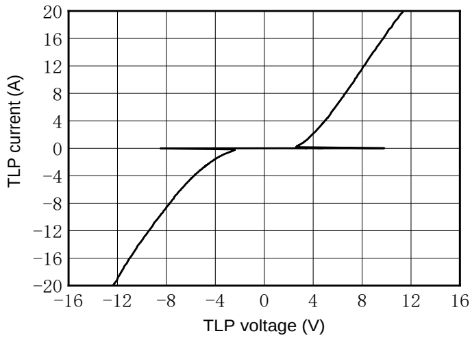
Fig. 7 TLP Measurement
