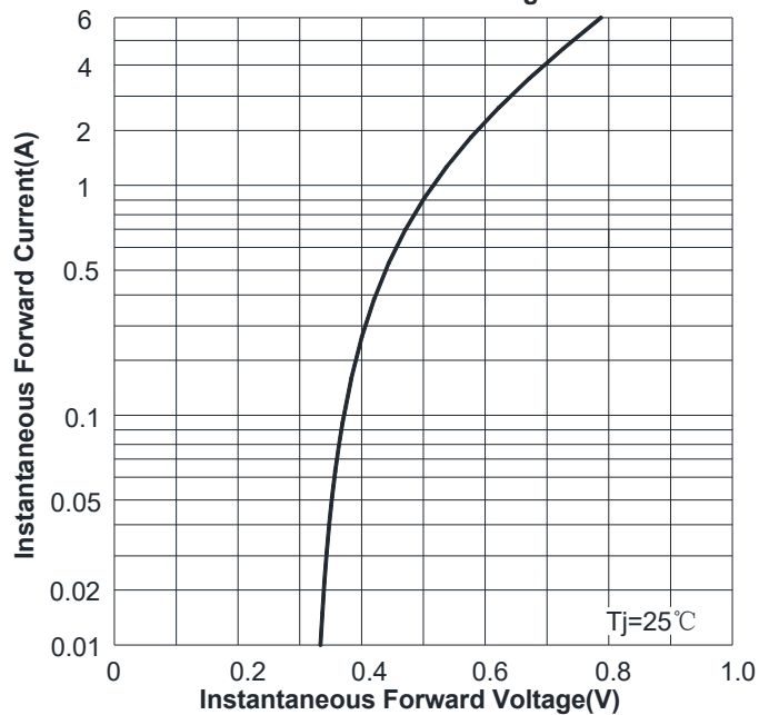
FIG3: Forward Voltage
