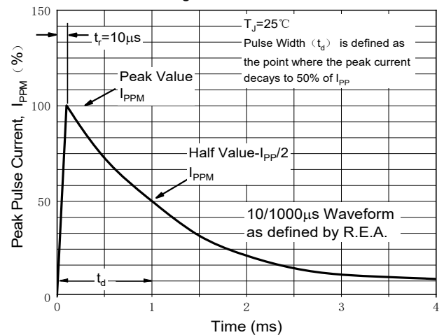
Fig.3 Pulse Waveform
