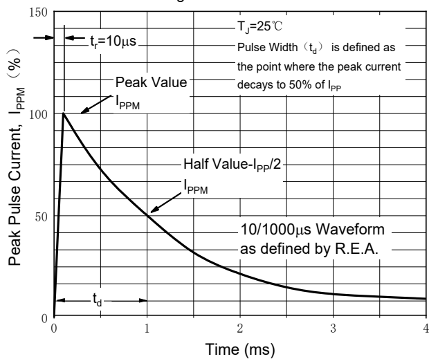
Fig.3 Pulse Waveform
