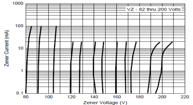
Fig. 4 - Typical Zener Breakdown Characteristics
