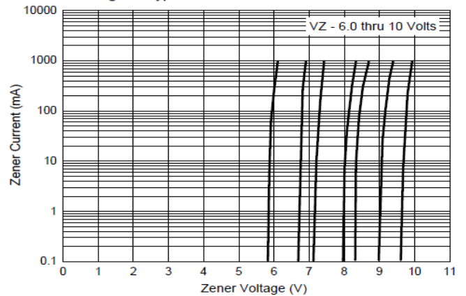
Fig. 2 - Typical Zener Breakdown Characteristics
