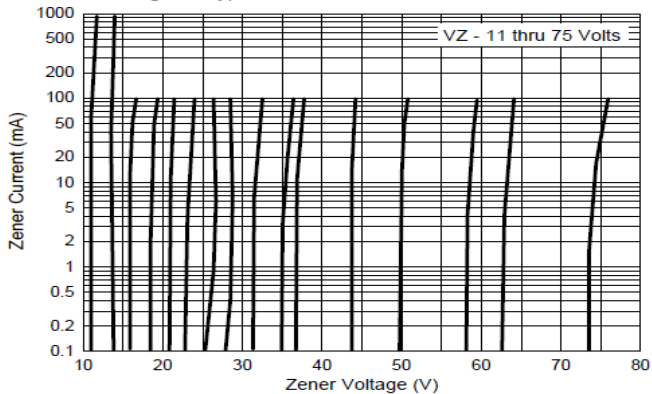
Fig. 3 - Typical Zener Breakdown Characteristics
