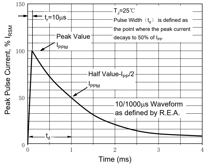
Fig.2 Pulse Waveform
