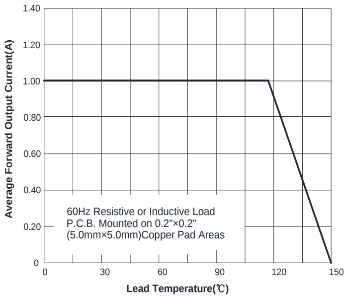
FIG.1: Io-TL Curve
