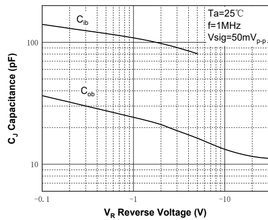
Fig.6 - Capacitance
