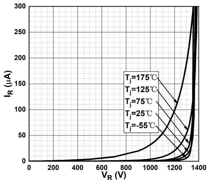
Figure 2. Reverse Characteristics
