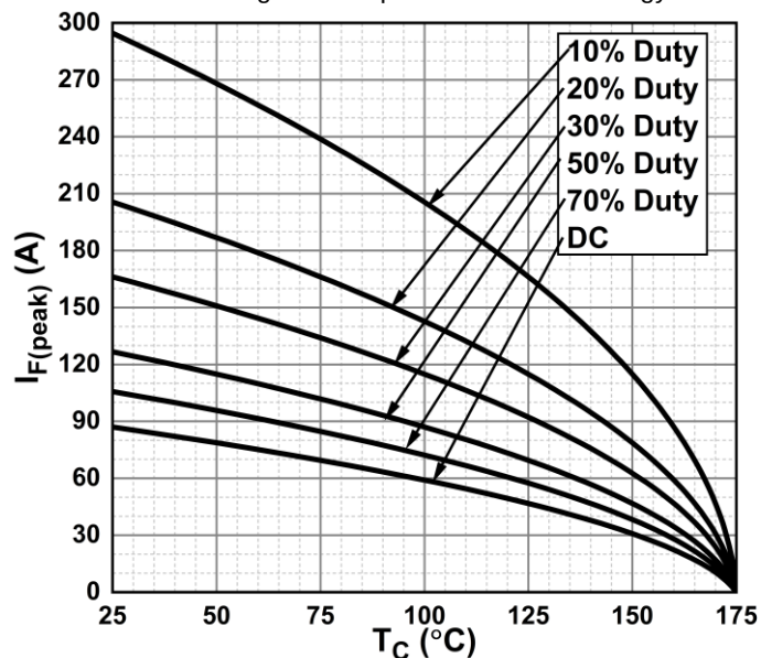
Figure 7. Current Derating
