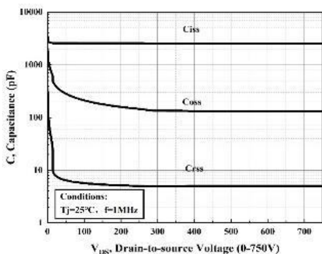
Figure 13. Capacitances vs. Drain Source Voltage (0-750V)
