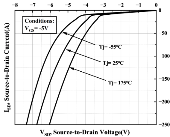
Figure 9. Body Diode Characteristic
