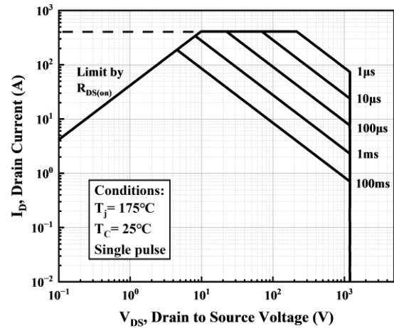
Figure 22. Safe Operating Area
