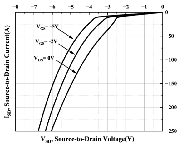
Figure 8. Body Diode Characteristic at T_j = 25^\circ\text{C}
