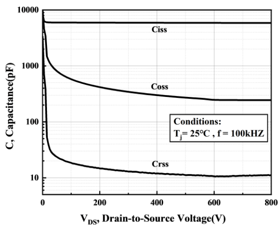
Figure 13. Capacitances vs. Drain Source Voltage (0-800V)
