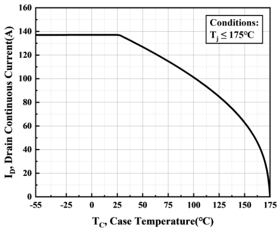
Figure 17. Continuous Drain Current Derating vs. Case Temperature
