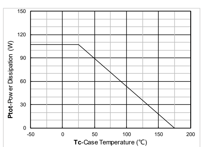
Figure 12. Power dissipation
