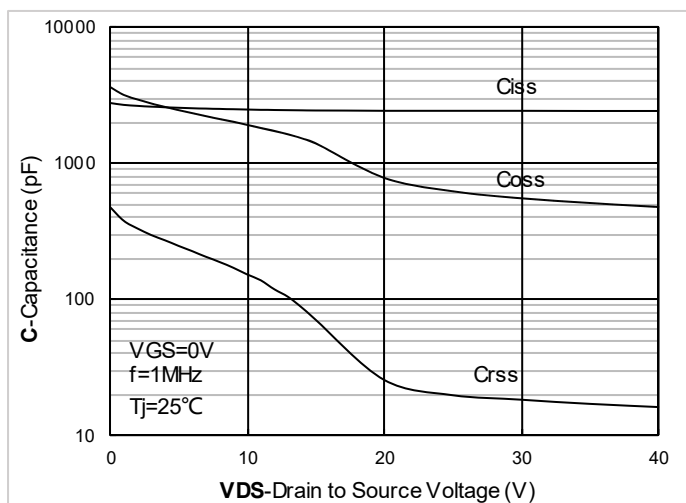
Figure 3. Capacitance Characteristics
