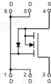
DFN2020-6L-WF
