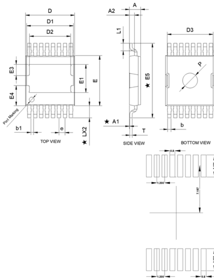
SUGGESTED SOLDER PAD LAYOUT
