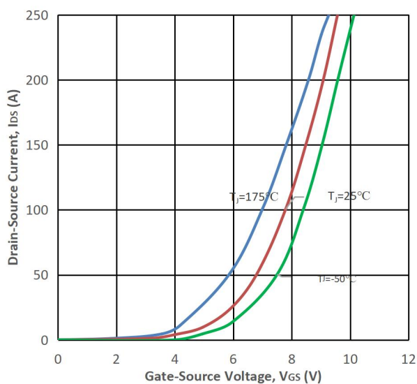
Fig5. Transfer Characteristic
