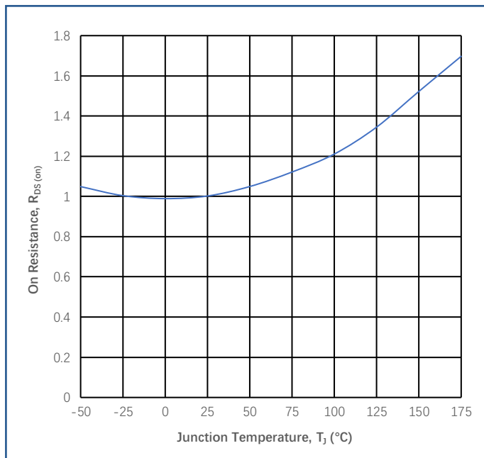
Figure 2 Normalized On-Resistance vs. T_J
