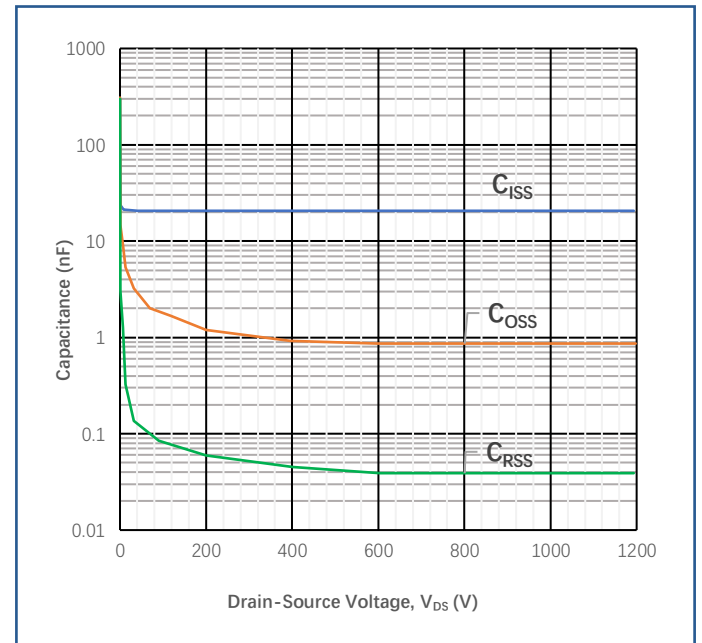
Figure 8 Capacitances vs. V_{DS}
