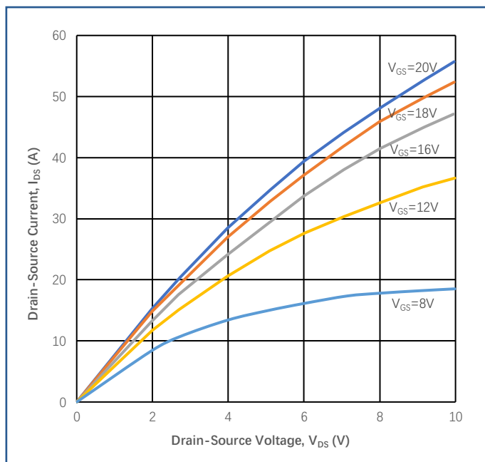
Figure 2 Output Characteristics (T J =175 °C)
