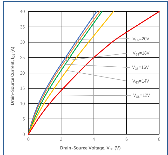
Figure 2 Output Characteristics ( T_J = 150^\circ\text{C} )
