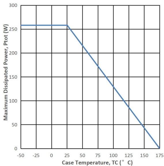
Fig12. Max Power Dissipation Derating Vs Tc
