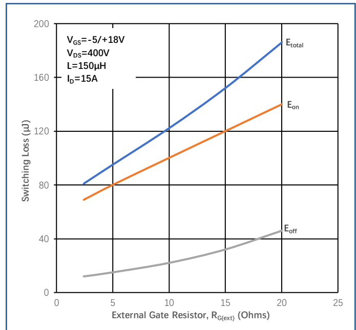
Figure 14 Switching Energy vs. R_{\text{G(ext)}}
