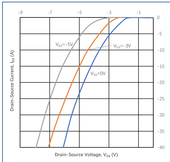
Figure 6 Body Diode Characteristic at 25^\circ\text{C}
