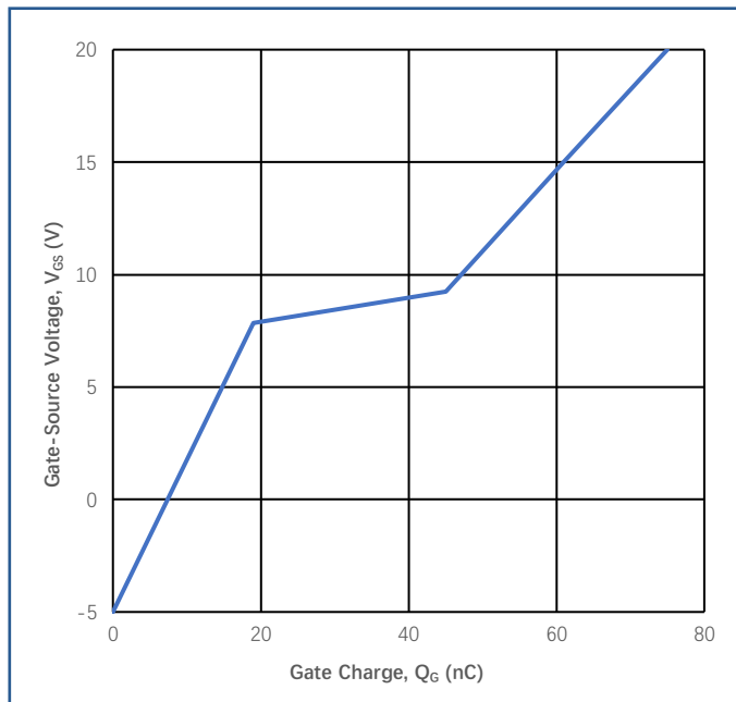
Figure 8 Gate Charge Characteristics
