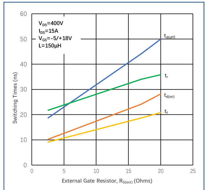
Figure 16 Switching Times vs. R_{\text{G(ext)}}
