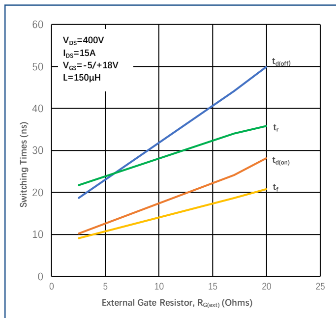
Figure 16 Switching Times vs. R_{\text{G(ext)}}
