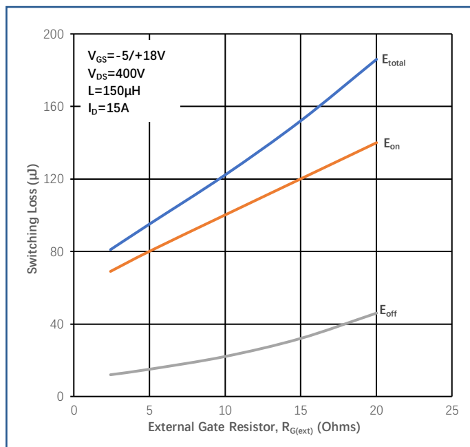
Figure 14 Switching Energy vs. R_{\text{G(ext)}}
