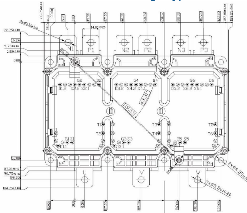
Package Type: HPD
