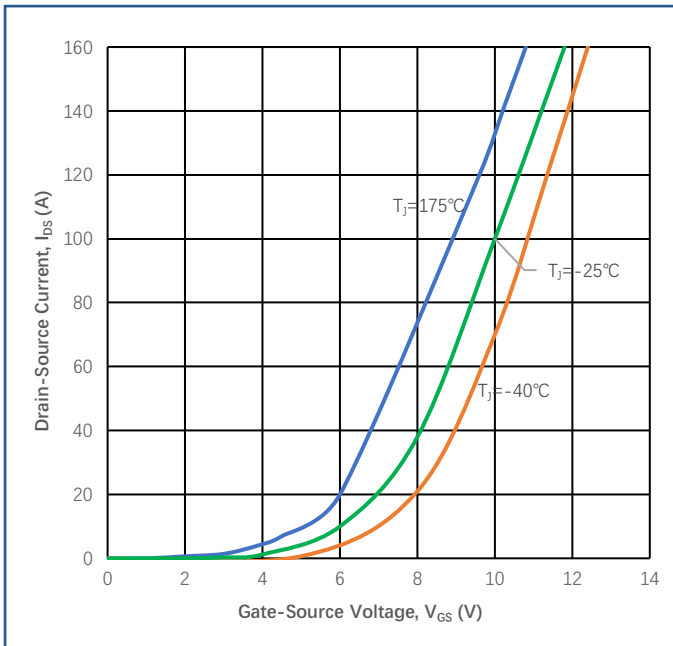
Figure 5 Transfer Characteristic
