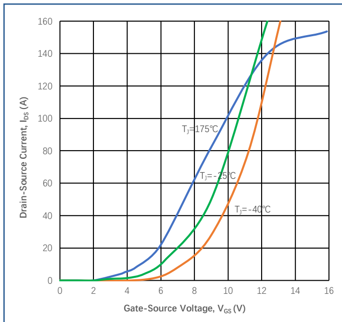
Figure 5 Transfer Characteristic
