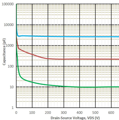
Fig11. Capacitances vs. Drain-Source
