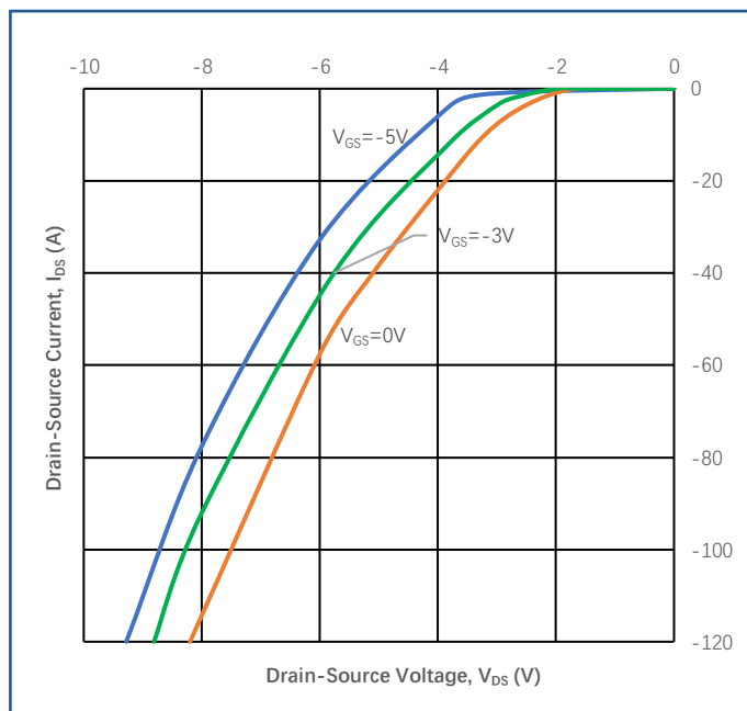
Figure 6 Body Diode Characteristic at 25^\circ C
