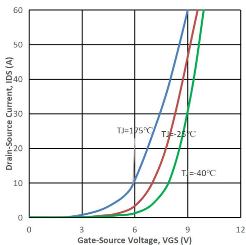
Fig5. Transfer Characteristic
