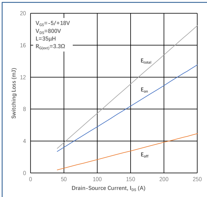
Figure 9 Inductive Switching Energy vs. Drain Current
