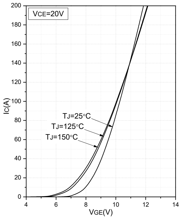
Fig.3 Transfer Characteristics
