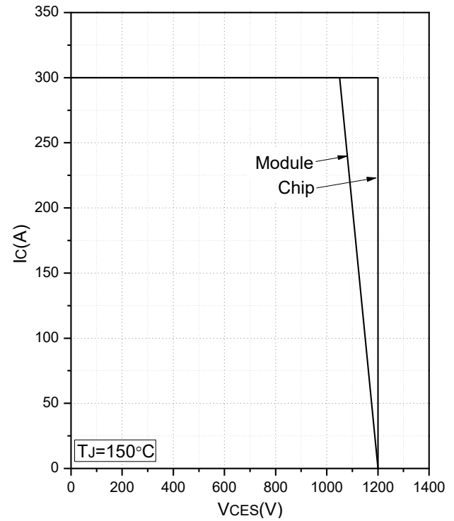
Fig.14 Reverse Bias Safe Operation Area (RBSOA)
