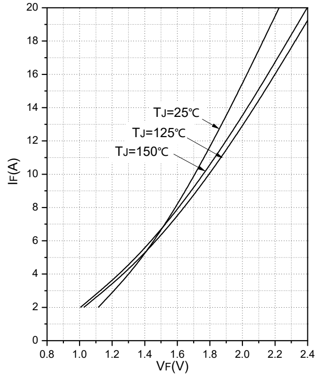
Fig.13 Typical Saturation Voltage Characteristics (Brake-Chopper) Fig.14 Forward Characteristics of Diode (Brake-Chopper)
