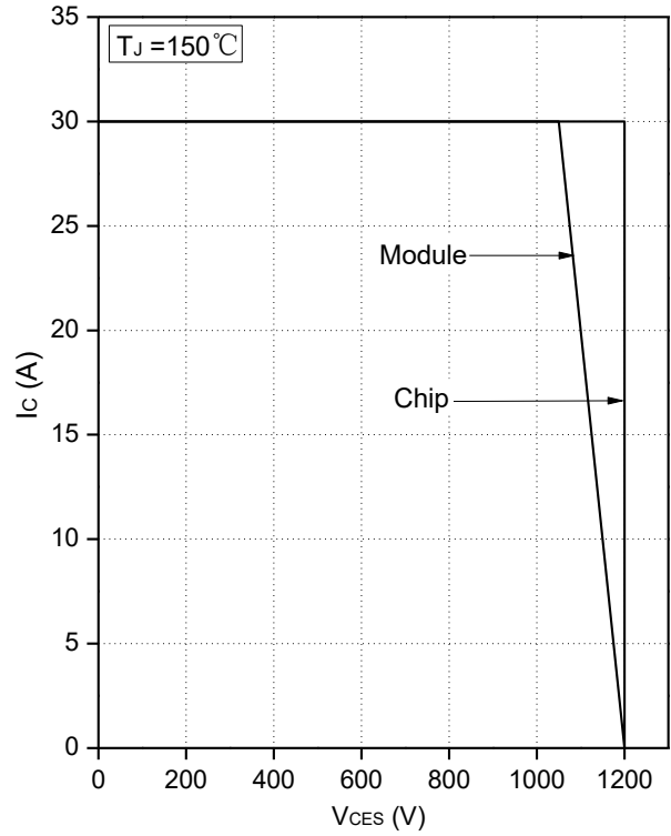
Fig.10 Reverse Bias Safe Operation Area (Inverter)
