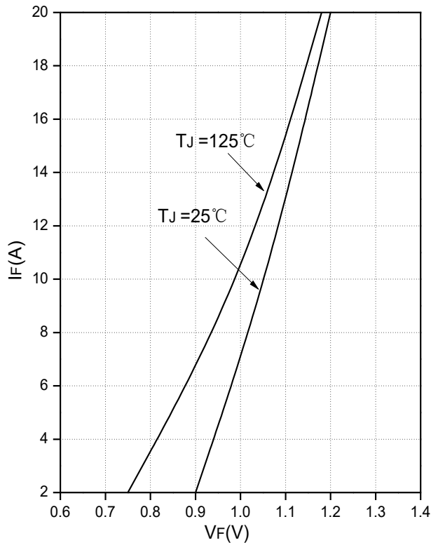
Fig.15 Forward Characteristics of Diode (Rectifier)
