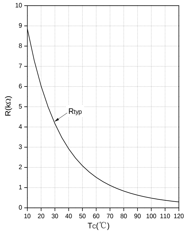
Fig.16 NTC Temperature Characteristics
