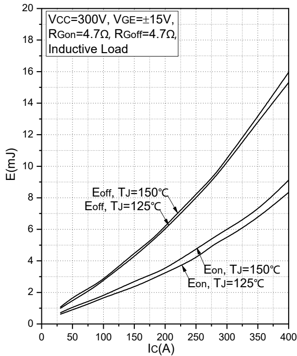
Fig.3 Typical Switching Loss vs. Collector Current
