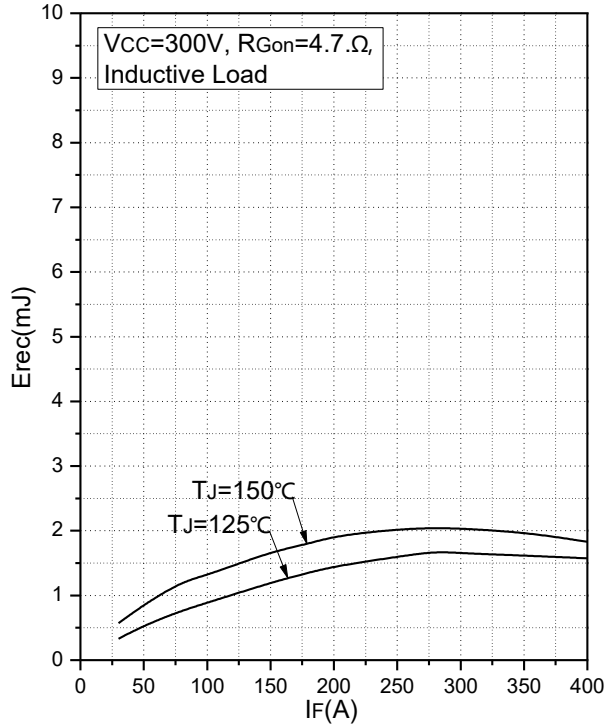
Fig.5 Typical Switching Loss vs. Forward Current
