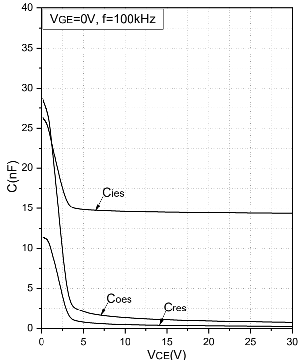
Fig.10 Capacitance Characteristics
